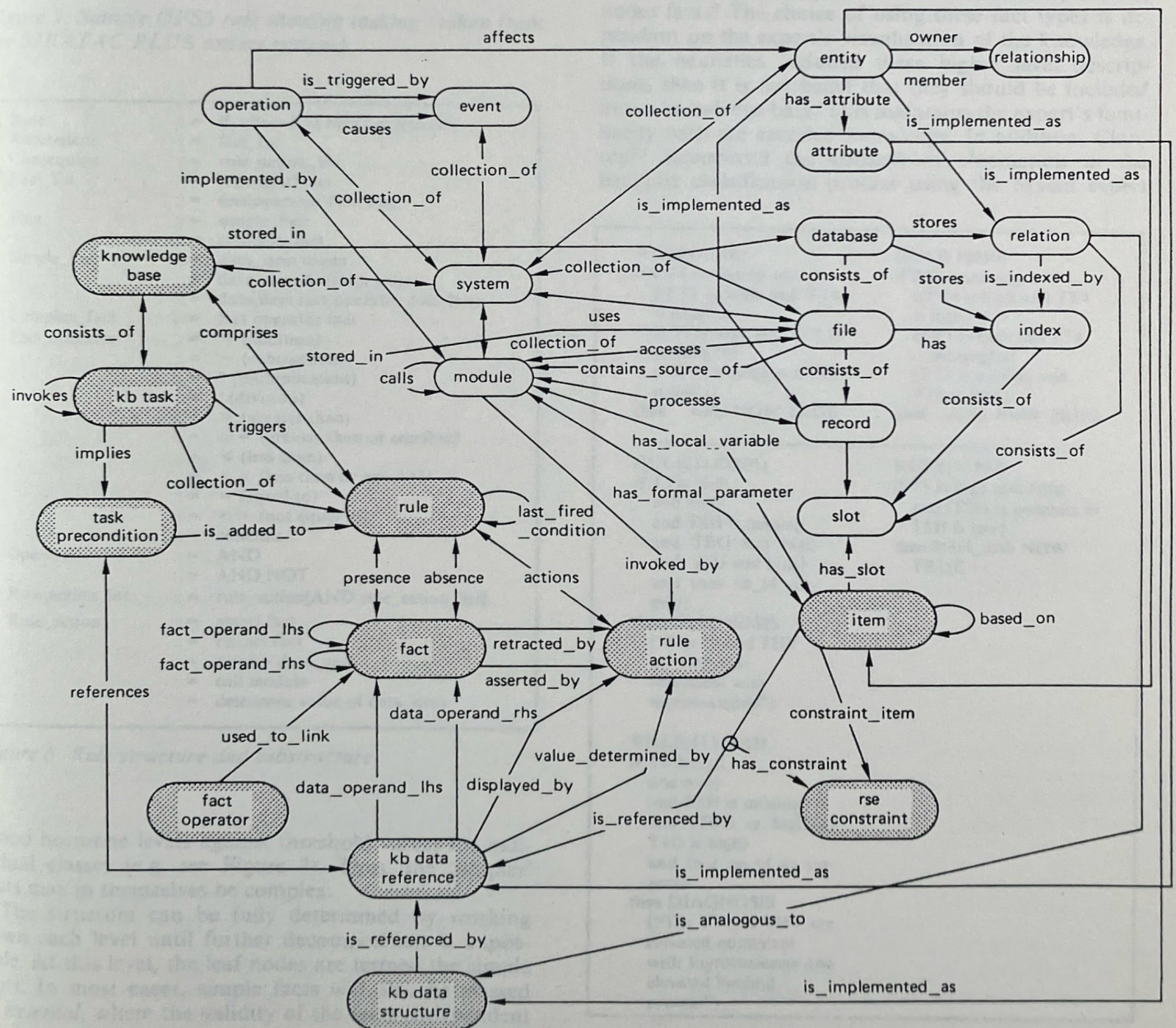
Figure 4. Knowledge dictionary conceptual model
