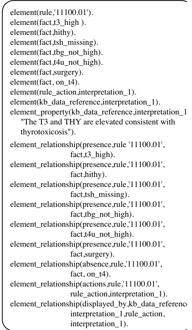
Figure 3.2 - Example of object and relationship storage in the Knowledge Dictionary
