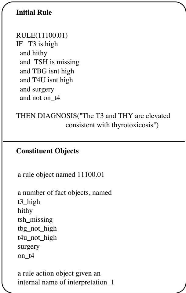
Figure 3.1 - An example rule, showing its decomposition into constituent objects 6
